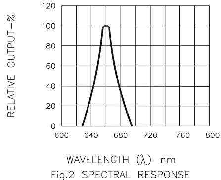
Fig.2 SPECTRAL RESPONSE
